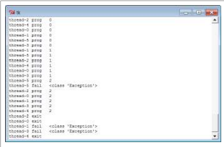
Figure 10-12. Messages from queued callbacks
