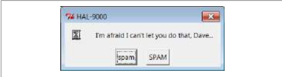
Figure 8-17. Old-style dialog
